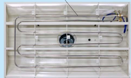
不鏽鋼蒸汽加熱管 Stainless steel steam heating pipe
